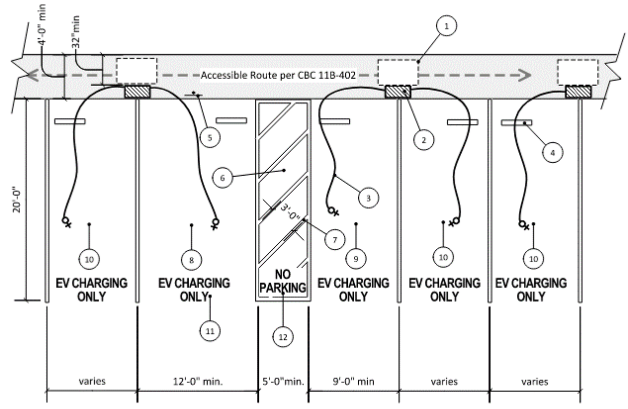
Typical Electric Vehicle Charging Station Configuration for Public Use
